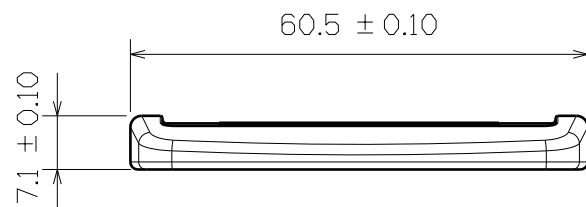
BOTTOM VIEW
