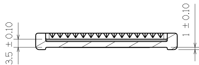
SECTION VIEW
